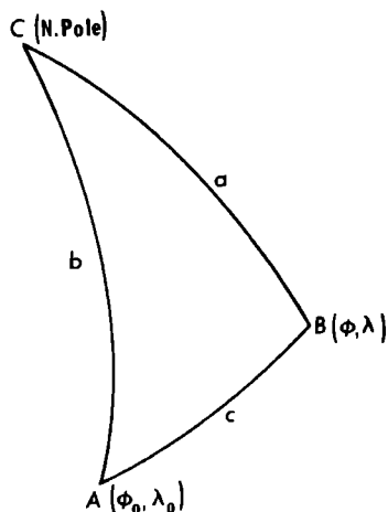
FIGURE 5.—Spherical triangle.
